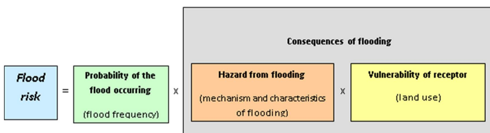
Figure 2 Conceptual definition of flood risk
